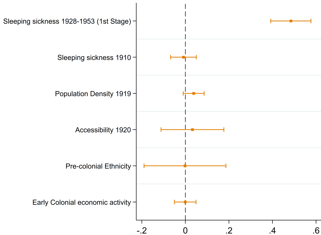
FIGURE 6: FALSIFICATION TESTS
